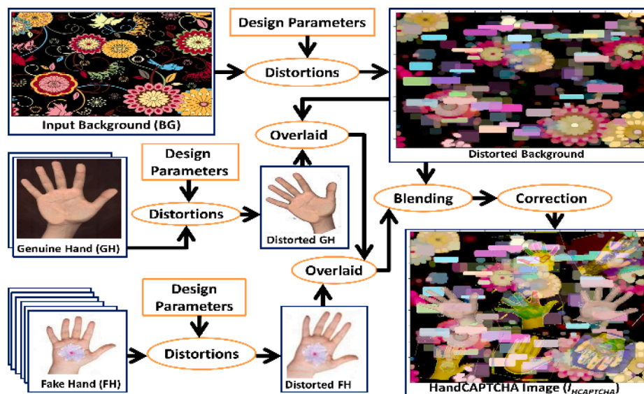
Fig. 2. Key steps of the HandCAPTCHA algorithm.
