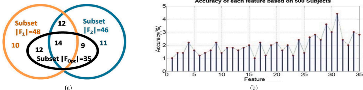
Fig. 9. (a) Feature subset formulation (Algorithm-2). (b) Performance evaluation of F_{Opt} by calculating the accuracy ( k -NN) of each feature independently.
