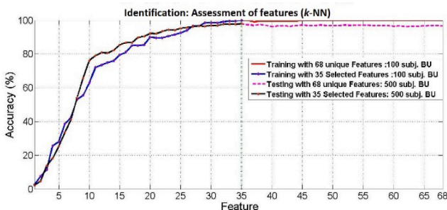
Fig. 10. (a) Feature-level assessment on F_3 for subset selection (Algorithm-2). (b) Identification performance evaluation of F_{Opt} using the k -NN and RF.
