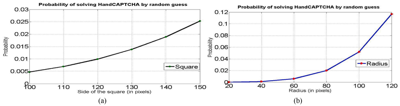
Fig. 6. Probability estimation of solving I_{HCAPTCHA} using different I_G dimensions by random guess-attacks. (a) I_G area: square. (b) I_G area: circle.
