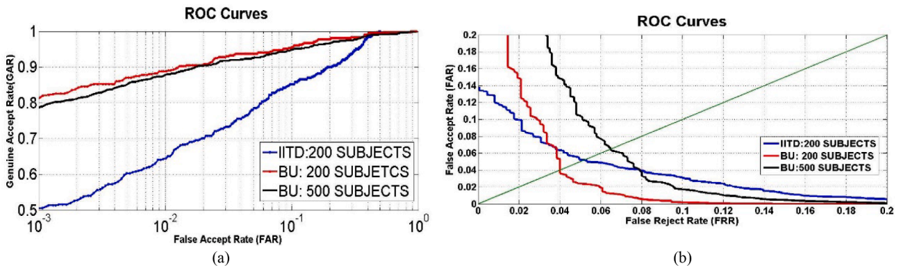
Fig. 13. ROC curves. (a) FAR vs. GAR is presented on the logarithmic scale for X-axis. (b) FRR vs. FAR for estimating EER using a diagonal line.
