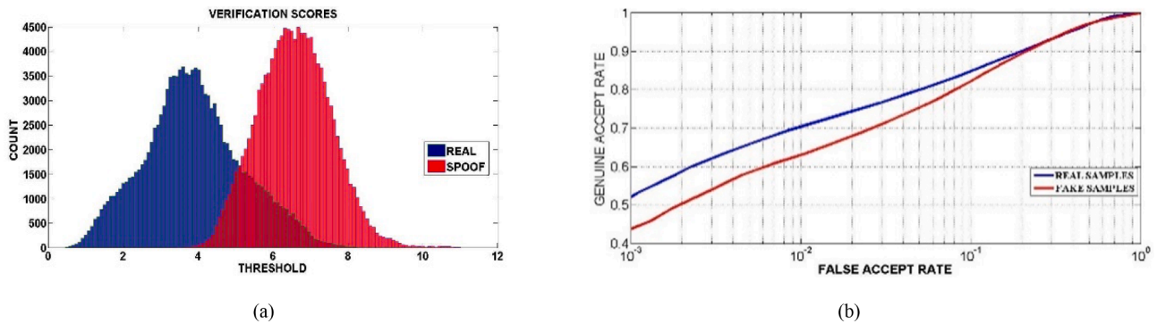
Fig. 8. (a). Verification score distribution of the real (blue) and fake (red) hands for IQ m . (b) The ROC curves are presented using the GAR and FAR.
