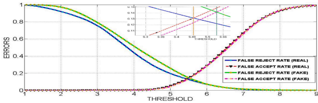
Fig. 7. Error estimation regarding the threshold during verification. A zoomed image in the inset implies the thresholds for EERs. For real samples, EER = 0.13 at th = 5.45 , and for fake samples, EER = 0.14 at th = 5.53 .
