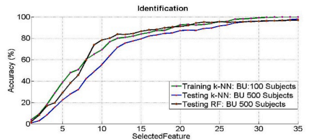
Fig. 10. (a) Feature-level assessment on F_3 for subset selection (Algorithm-2). (b) Identification performance evaluation of F_{Opt} using the k -NN and RF.
